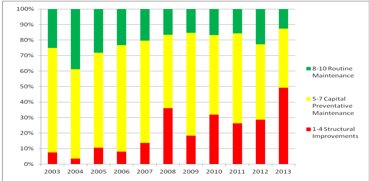
Figure 1: Percentage of federal-aid eligible road segments falling under surface condition classifications, by year, 2003-2013 for Berrien County
