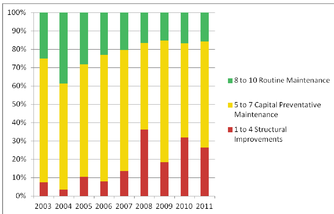
Figure 1: Percentage of road segments falling under surface condition classifications, by year
